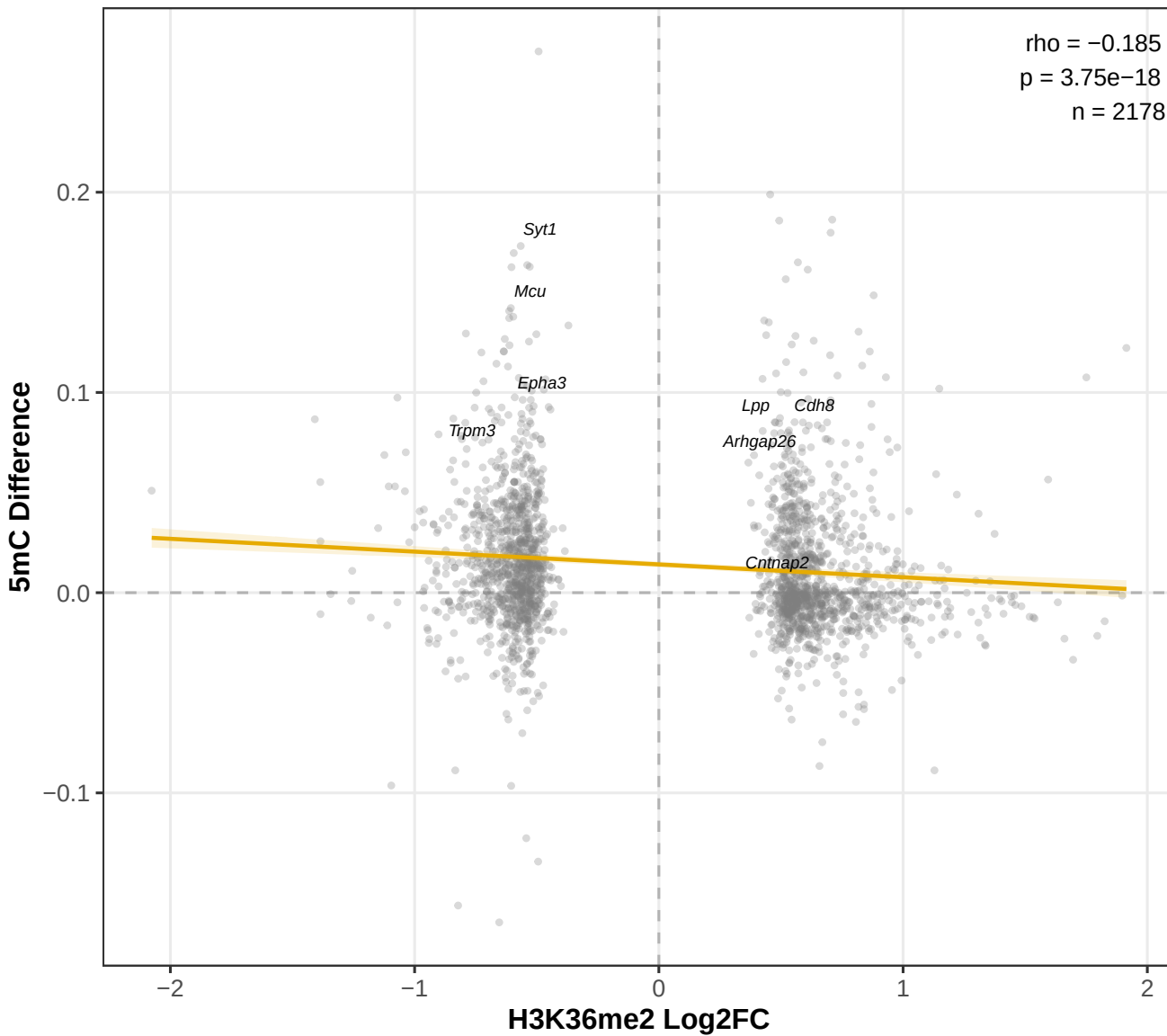
H3K36me2 Fold vs 5mC Change
