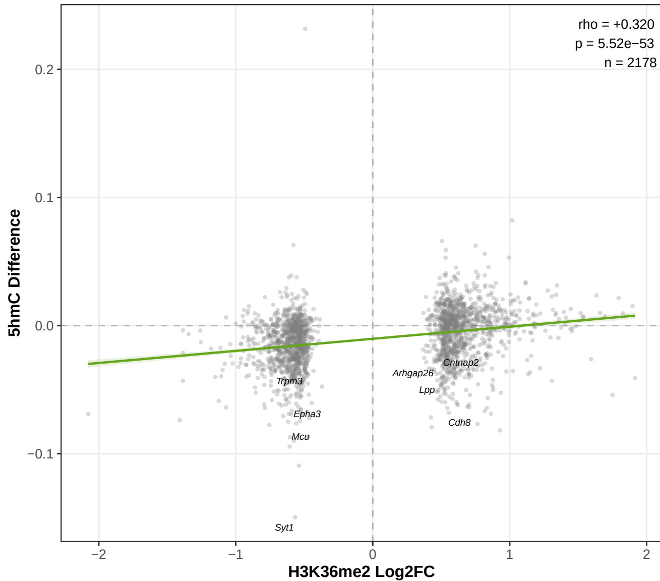
H3K36me2 Fold vs 5hmC Change
