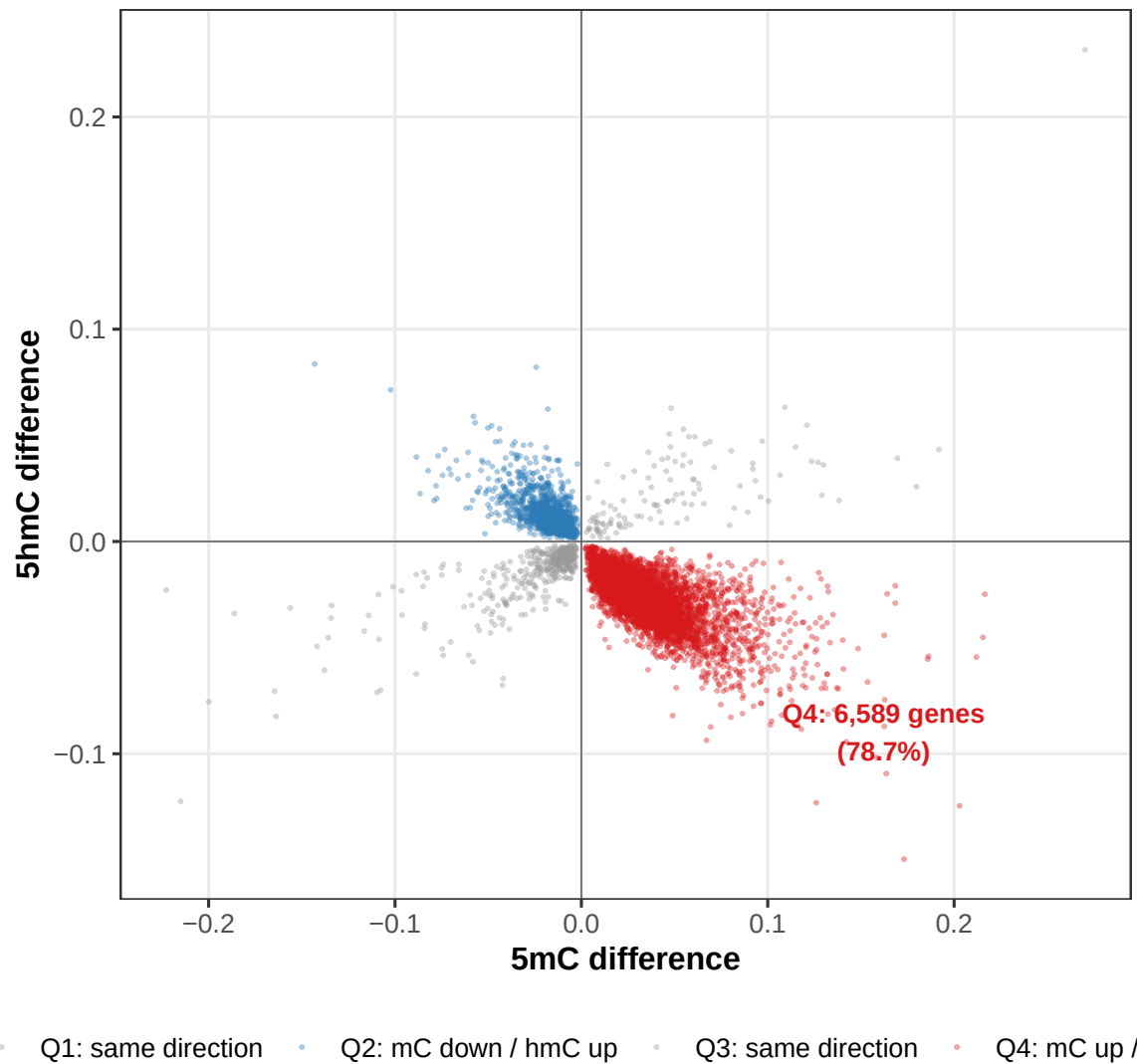
Co-significant genes: coordinated quadrant
