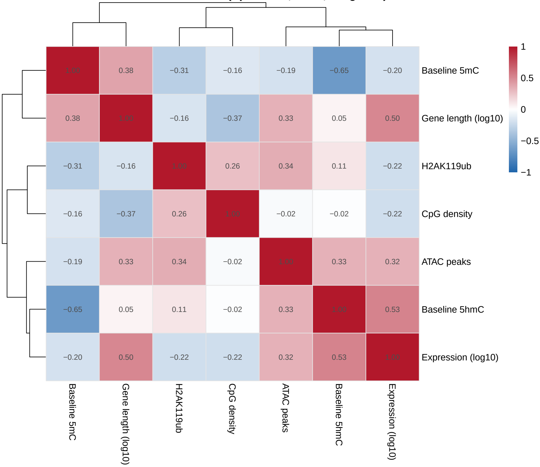
Feature Correlation Matrix (Spearman, N=11,937 genes)
