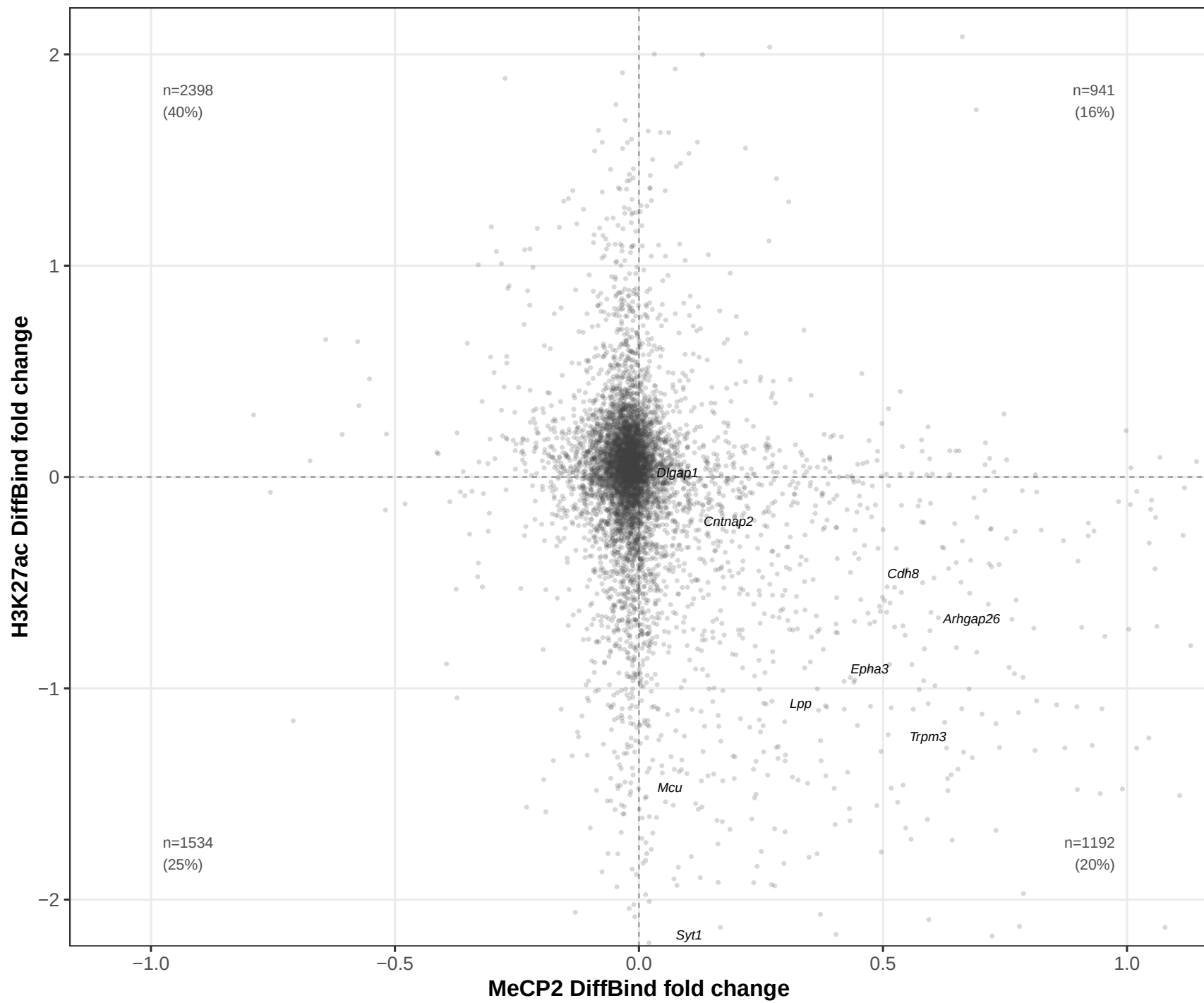
MeCP2 vs H3K27ac (Euchromatin Mark) Spearman rho = -0.211 , p < 2.2e-16 | n = 6,065 genes
