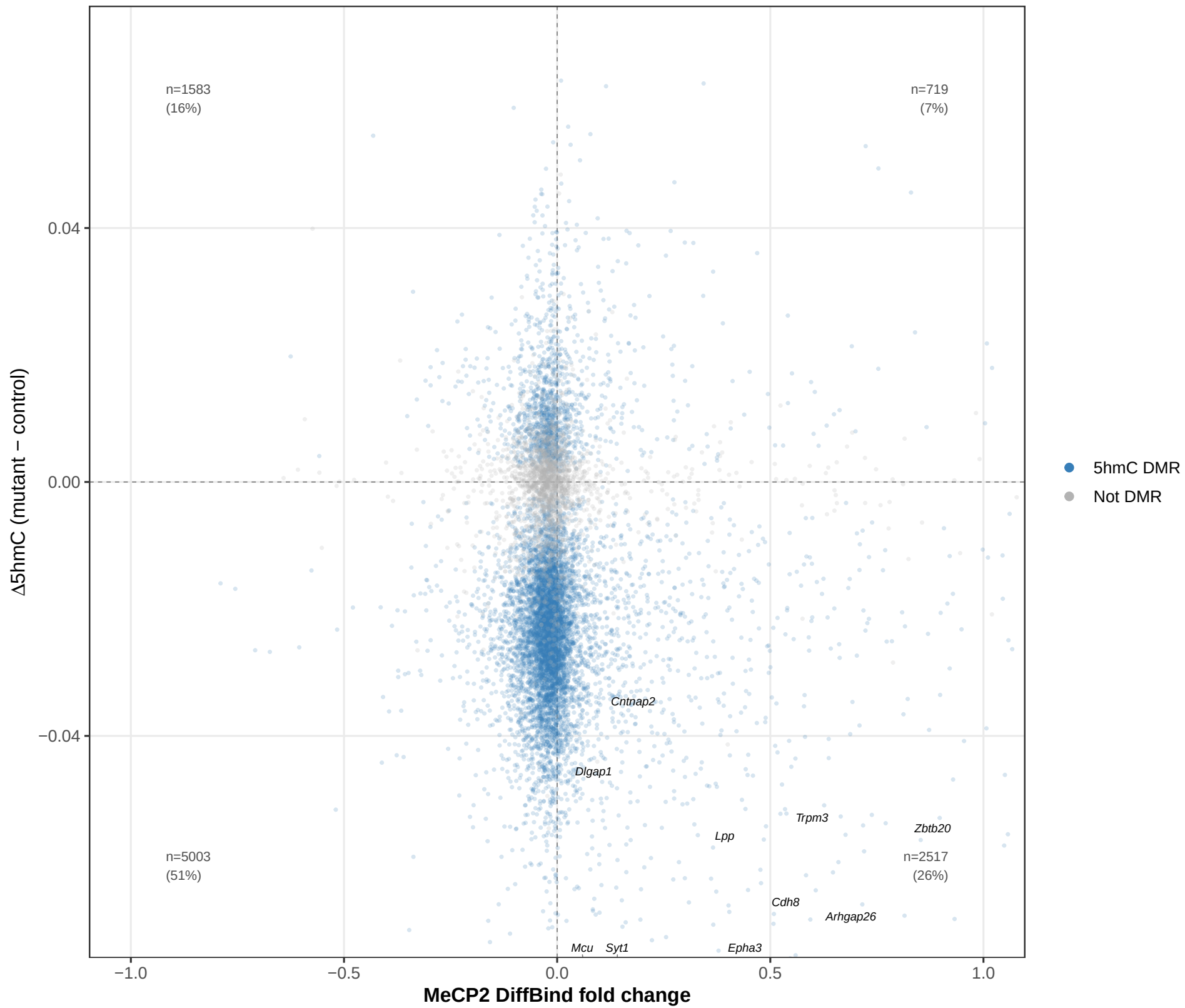
MeCP2 vs 5hmC Change at Gene Bodies Spearman rho = -0.040, p = 8.79e-05 | n = 9,822 genes
