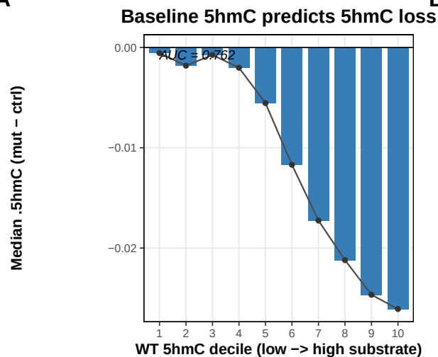
Figure 3. TET-impediment, not DNMT3A recruitment, drives BAP1-KO methylation remodeling
