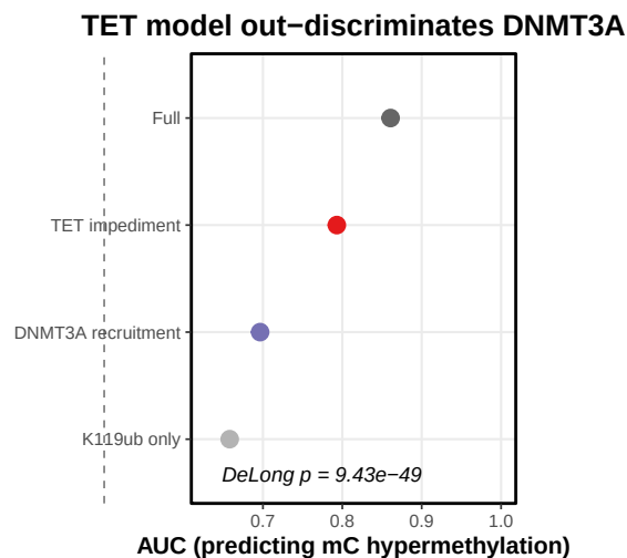
Figure 3. TET-impediment, not DNMT3A recruitment, drives BAP1-KO methylation remodeling
