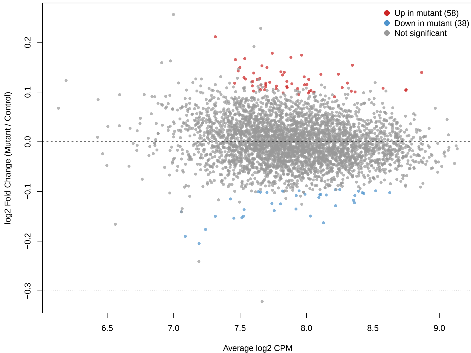
MA Plot – Stripenn Stripes (250831, 5kb)
