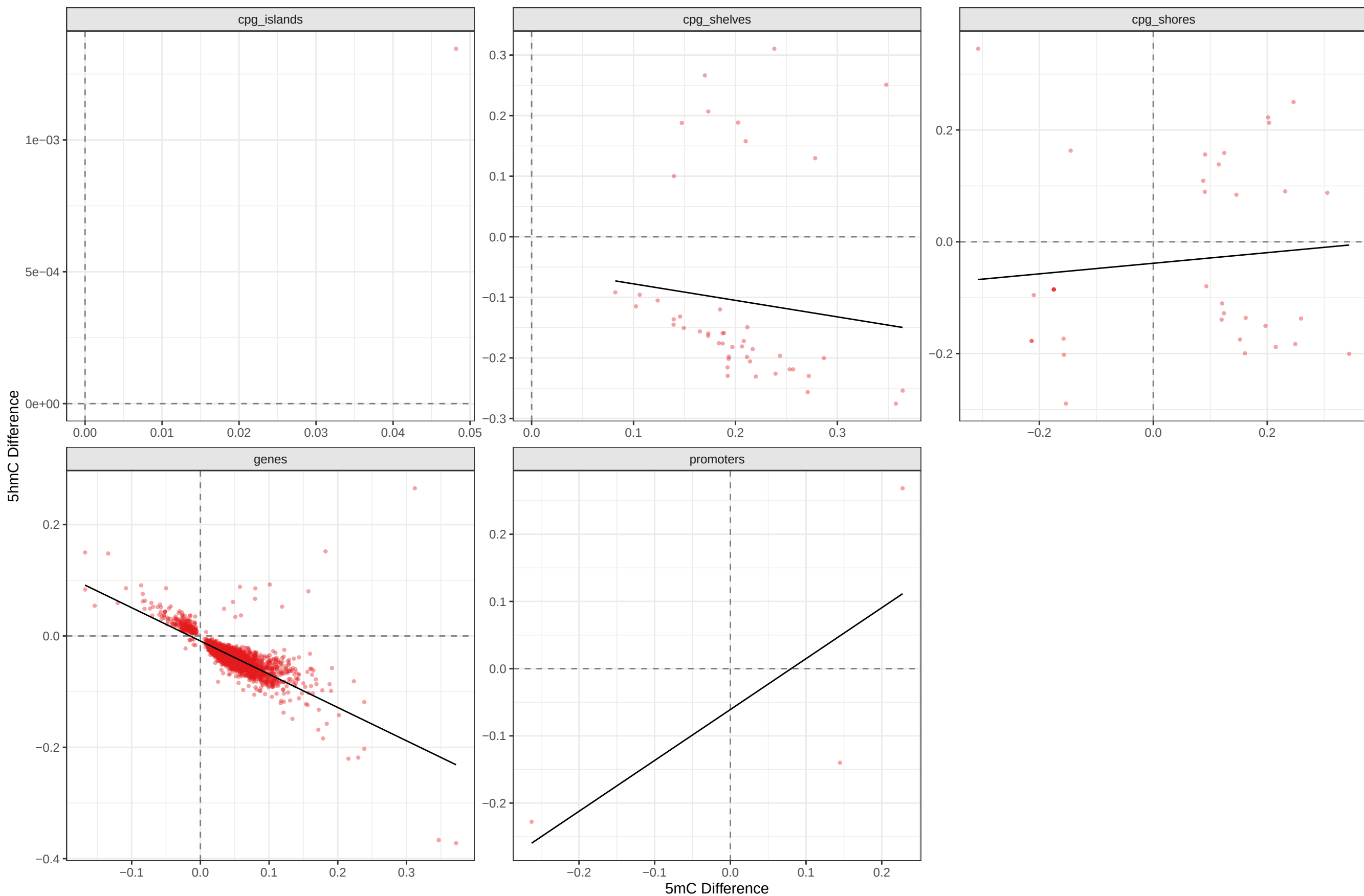
mC vs hmC Correlation by Annotation (CG Context)
