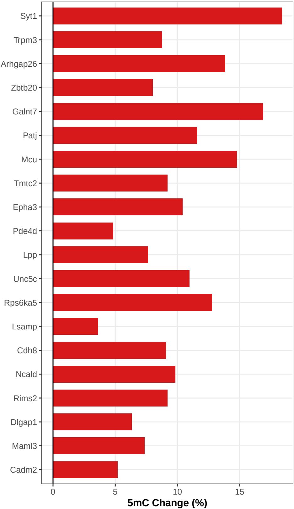
Top 20 Gene Body 5mC DMRs
