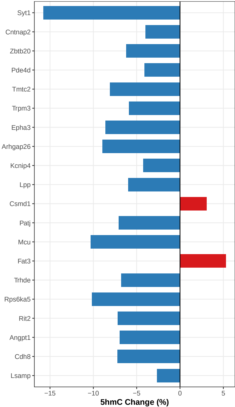
Top 20 Gene Body 5hmC DMRs
