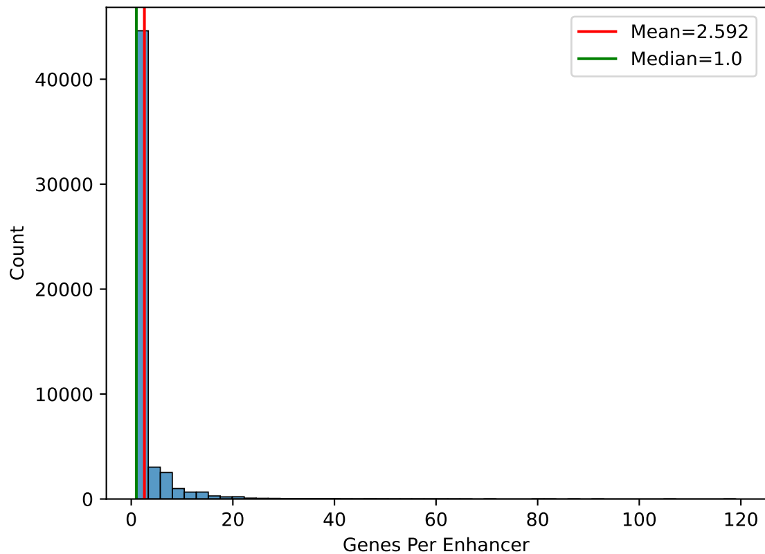
Number Of Genes Per Enhancer
