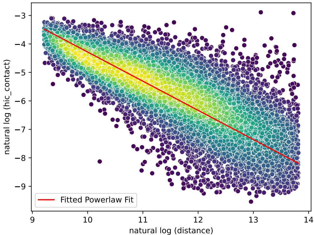
E-G Pair HiC Powerlaw Fit
