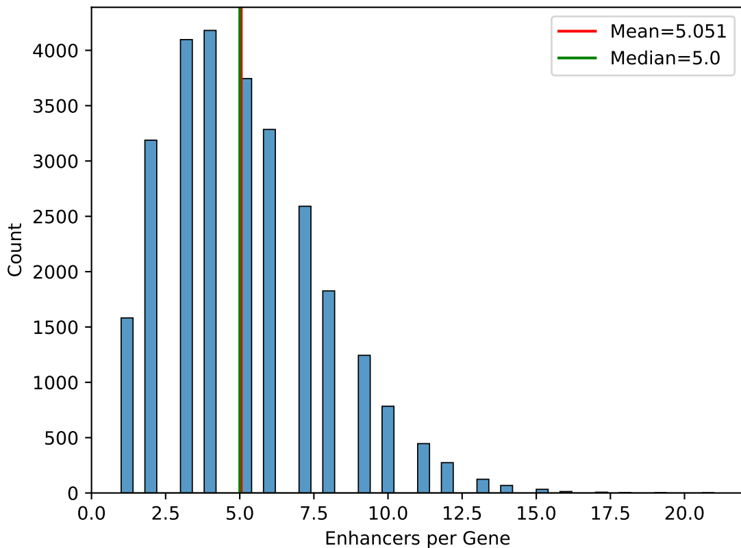
Number of Enhancers Per Gene
