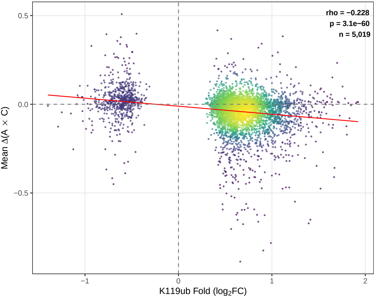
FDR < 0.05 only (rho = -0.228)
