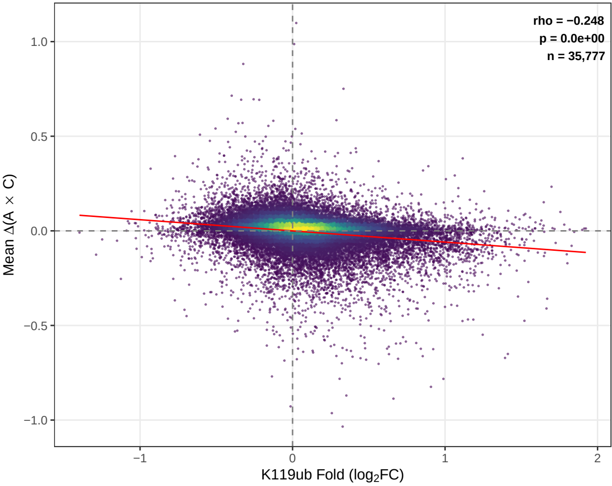
All enhancers (rho = -0.248)
