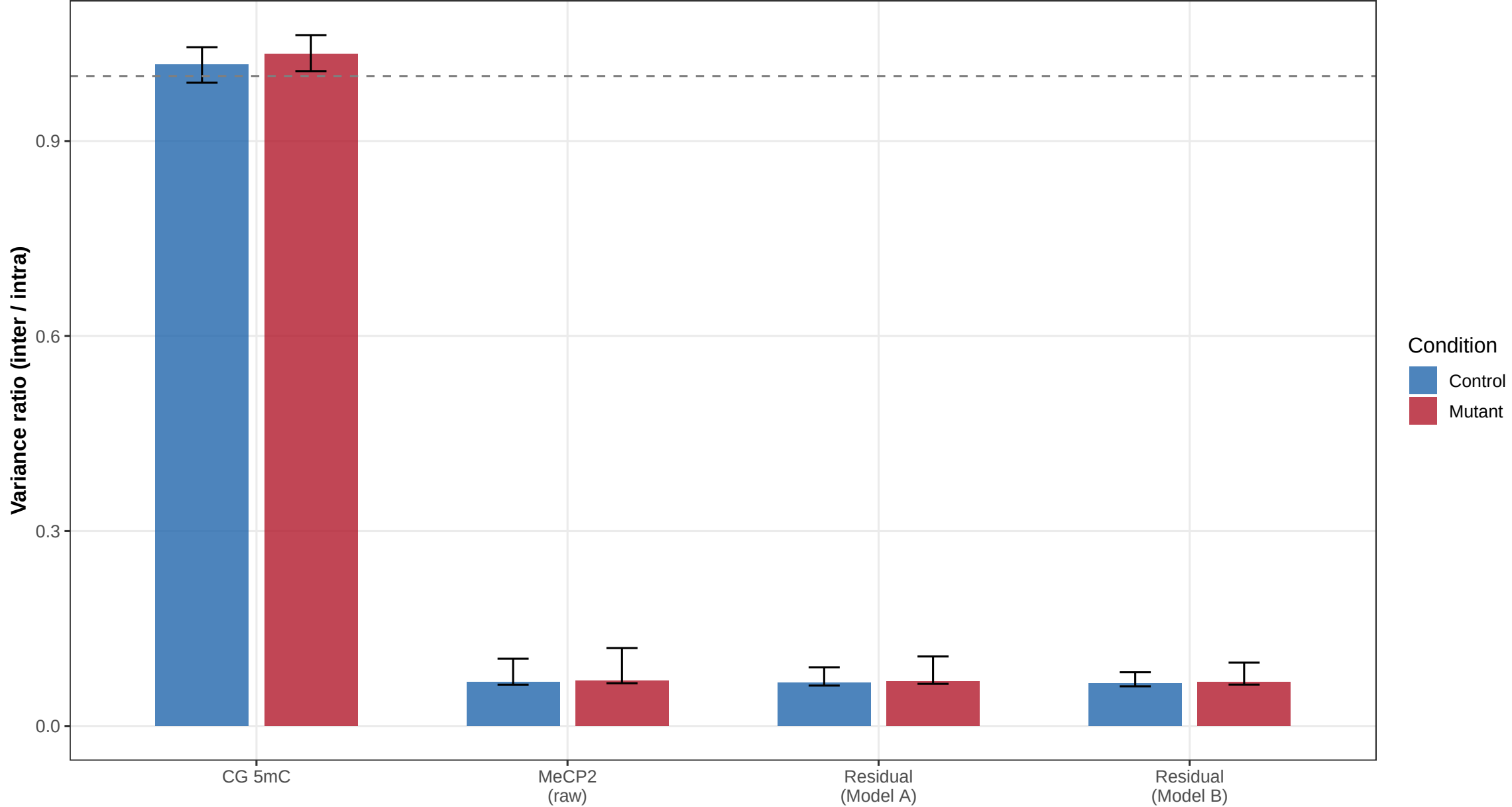
TAD Variance Ratios: Model A vs Model B Does including 5hmC in the correction change the result?
