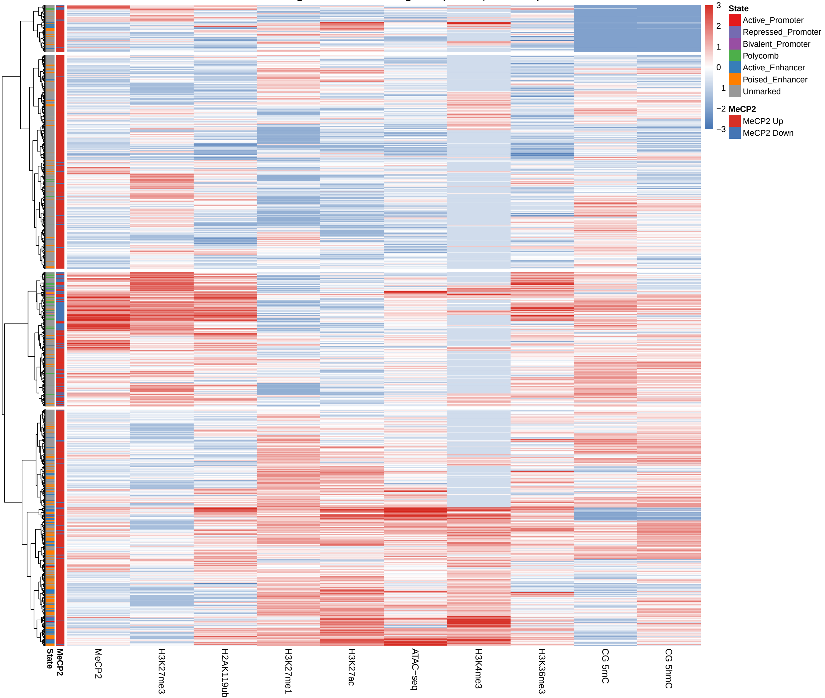
Multi-mark signal at MeCP2 binding sites (n=5000, Z-scored)
