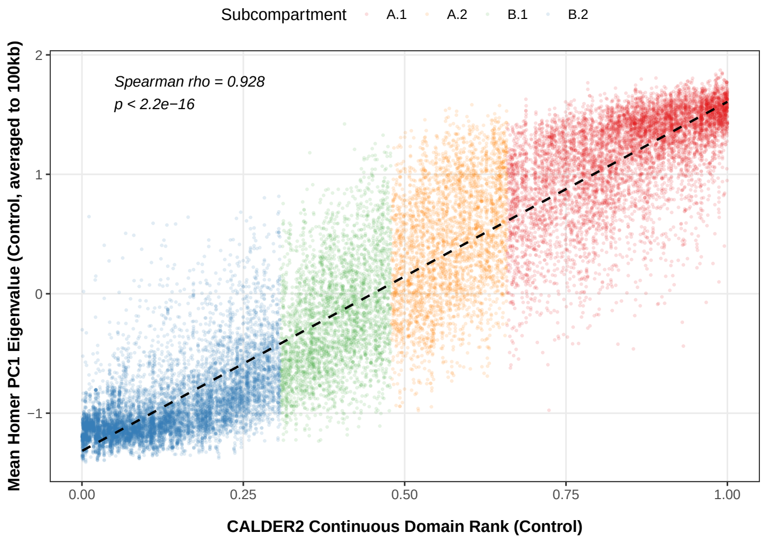
CALDER2 Continuous Domain Rank Distribution by Subcompartment Rank separation validates the 4-way classification (all KS p < 2.2e-16 )
