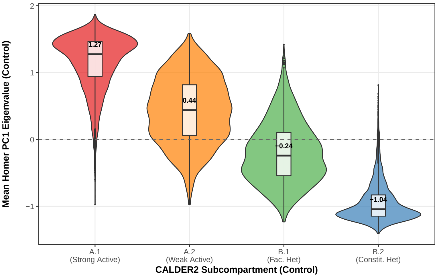
Concordance: CALDER2 vs Homer PC1 Compartment Classification Accuracy = 91.5% | Cohen's kappa = 0.829
