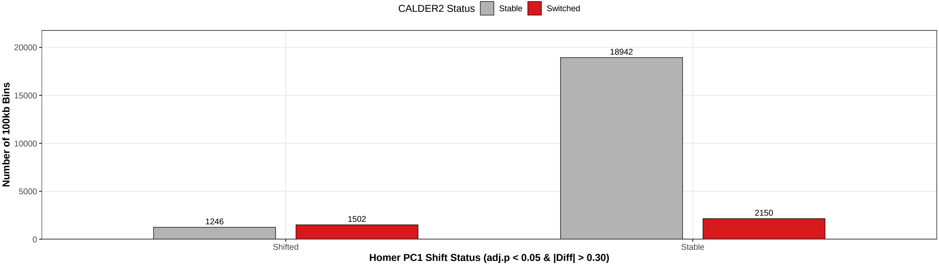
Compartment Switching Concordance: CALDER2 vs Homer Fisher's OR = 10.62, p < 2.2e-16 | Do the tools agree on which bins switch?
