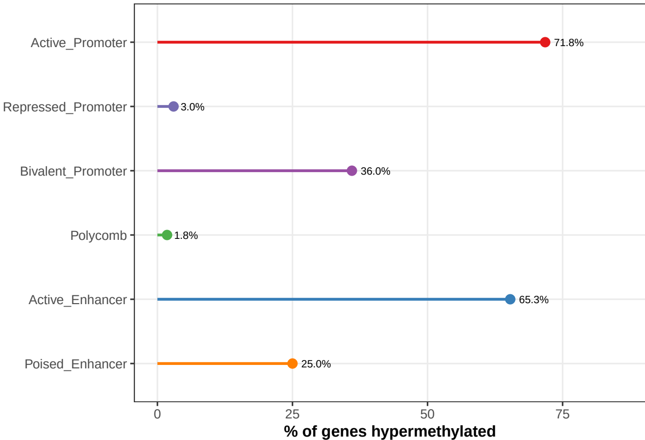
Active Promoter 72% vs Polycomb 1.8%
