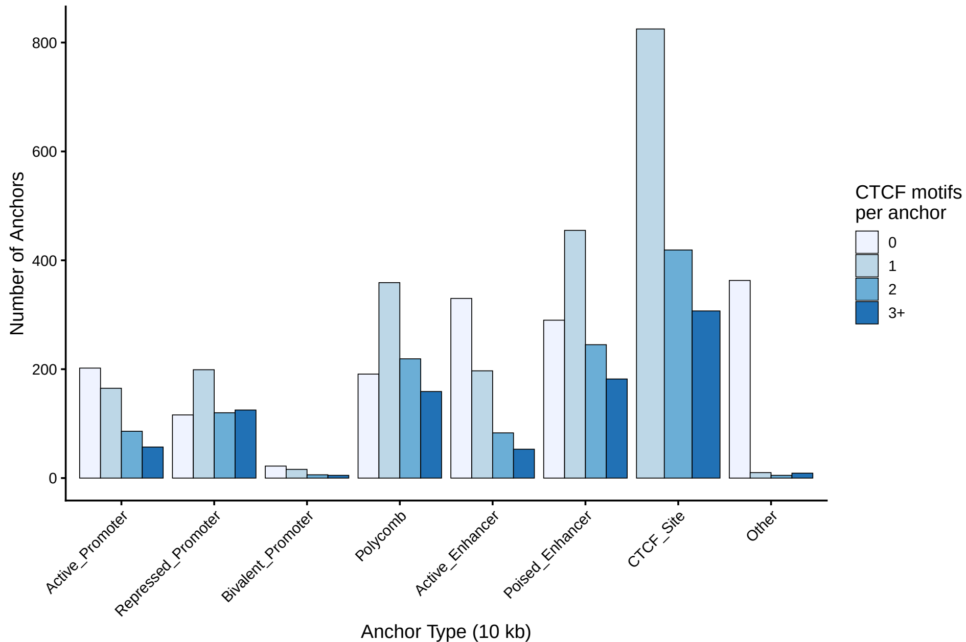
CTCF Motif Count per Anchor by Chromatin State
