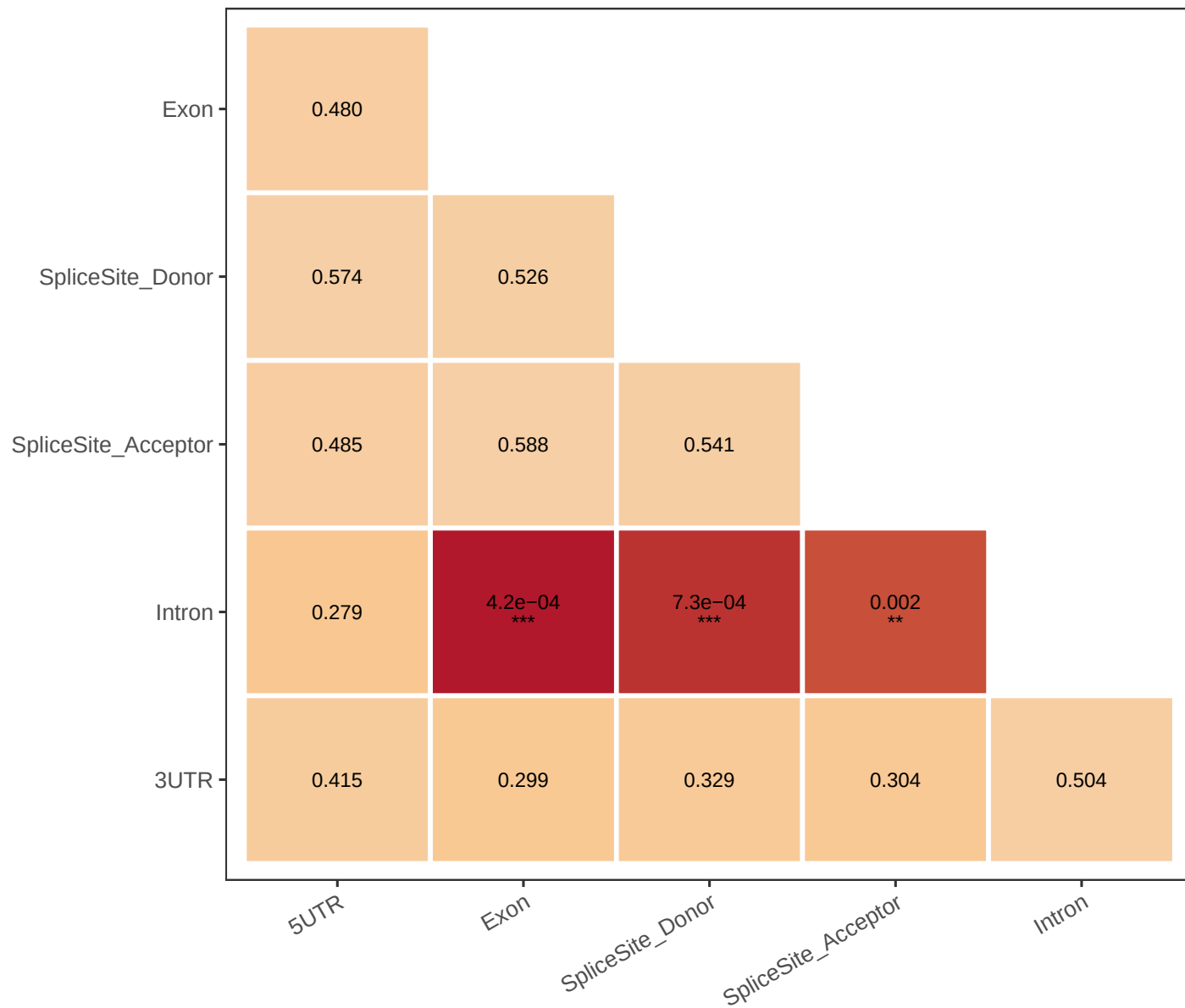
Dunn's Post-Hoc: \Delta 5mC
