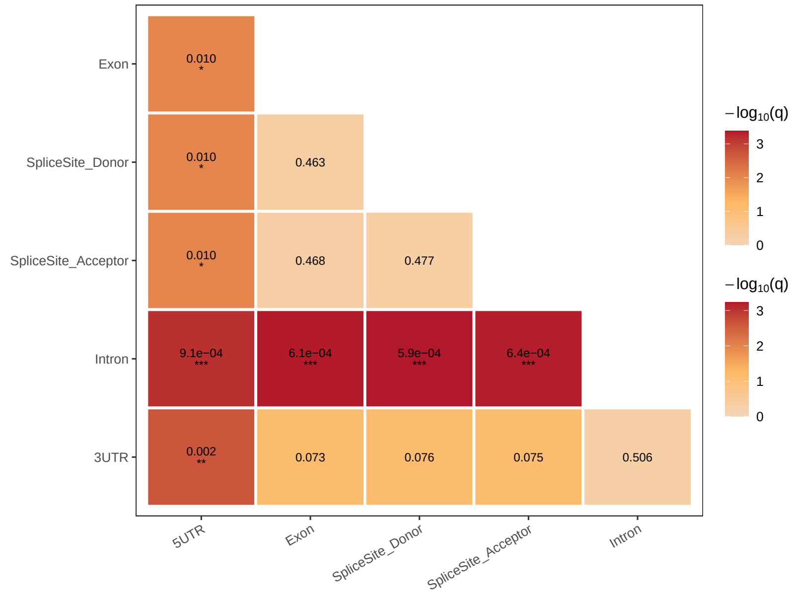
Dunn's Post-Hoc: \Delta 5hmC
