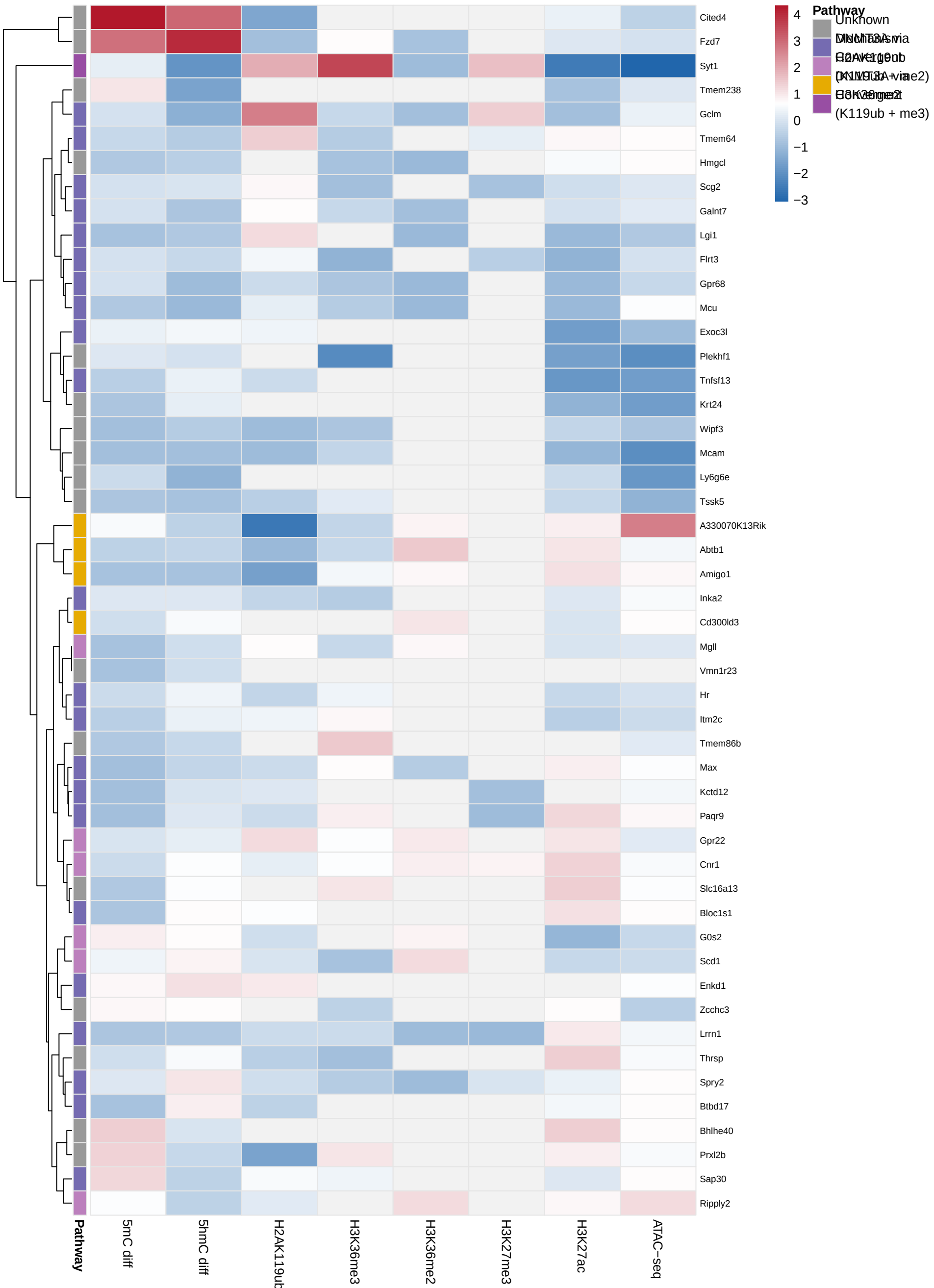
Top 50 Hypermethylated Genes: Multi-Mark Profile (Z-scored)
