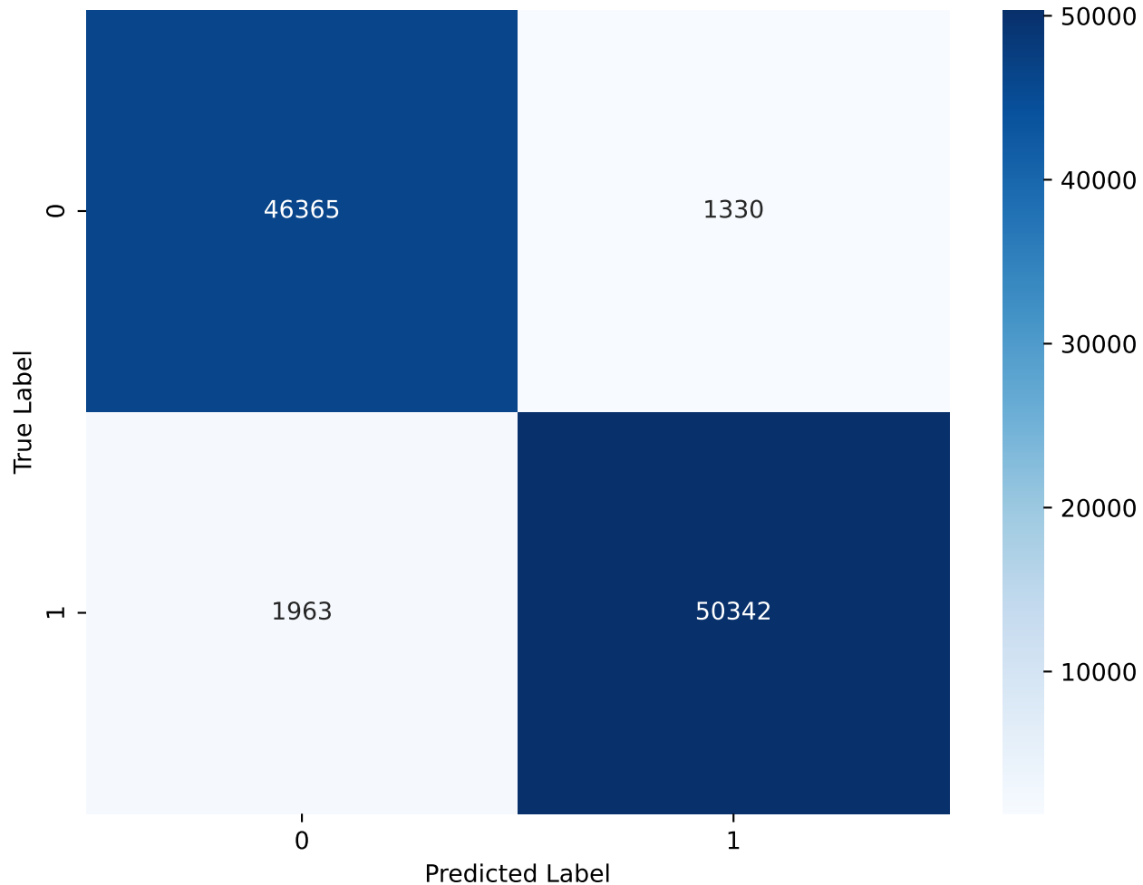
Confusion Matrix for Bilstm
