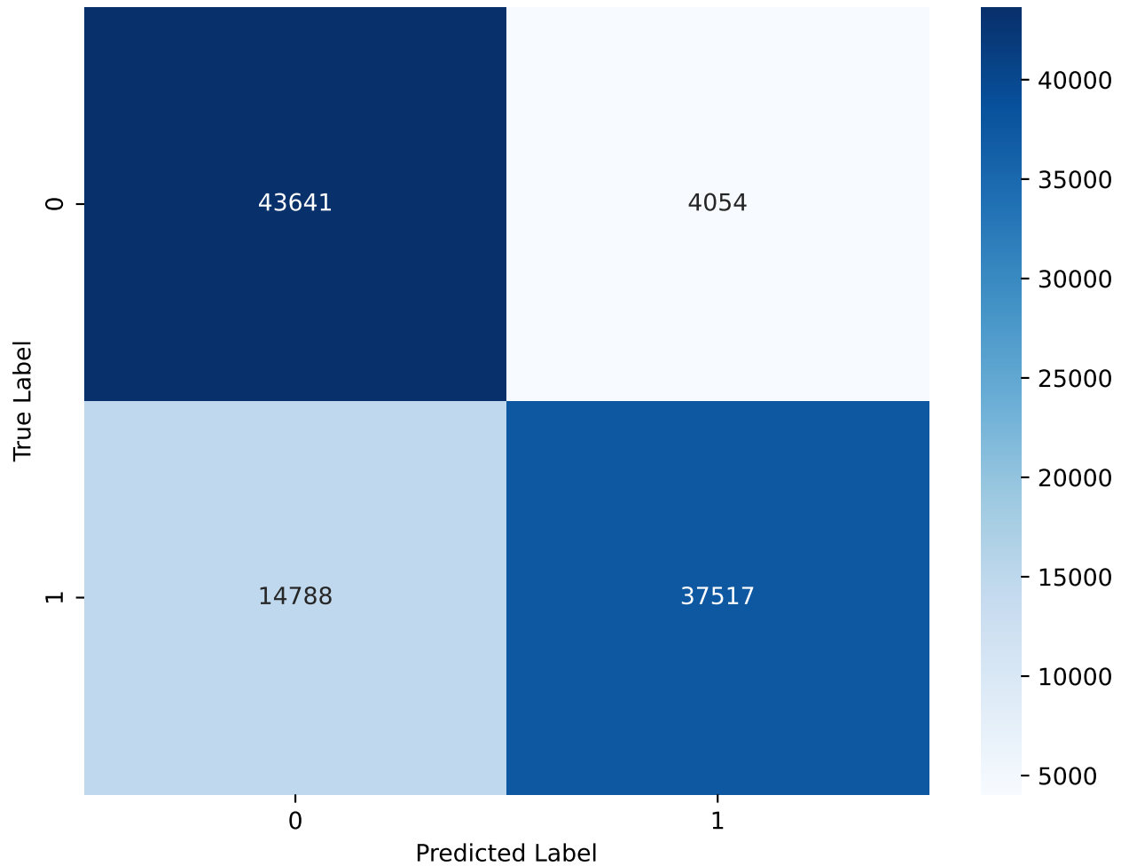
Confusion Matrix for D
