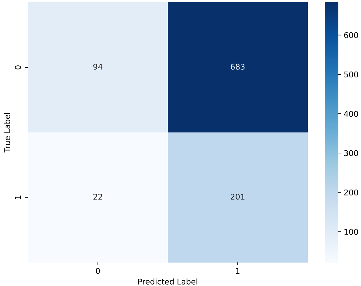
Confusion Matrix for A
