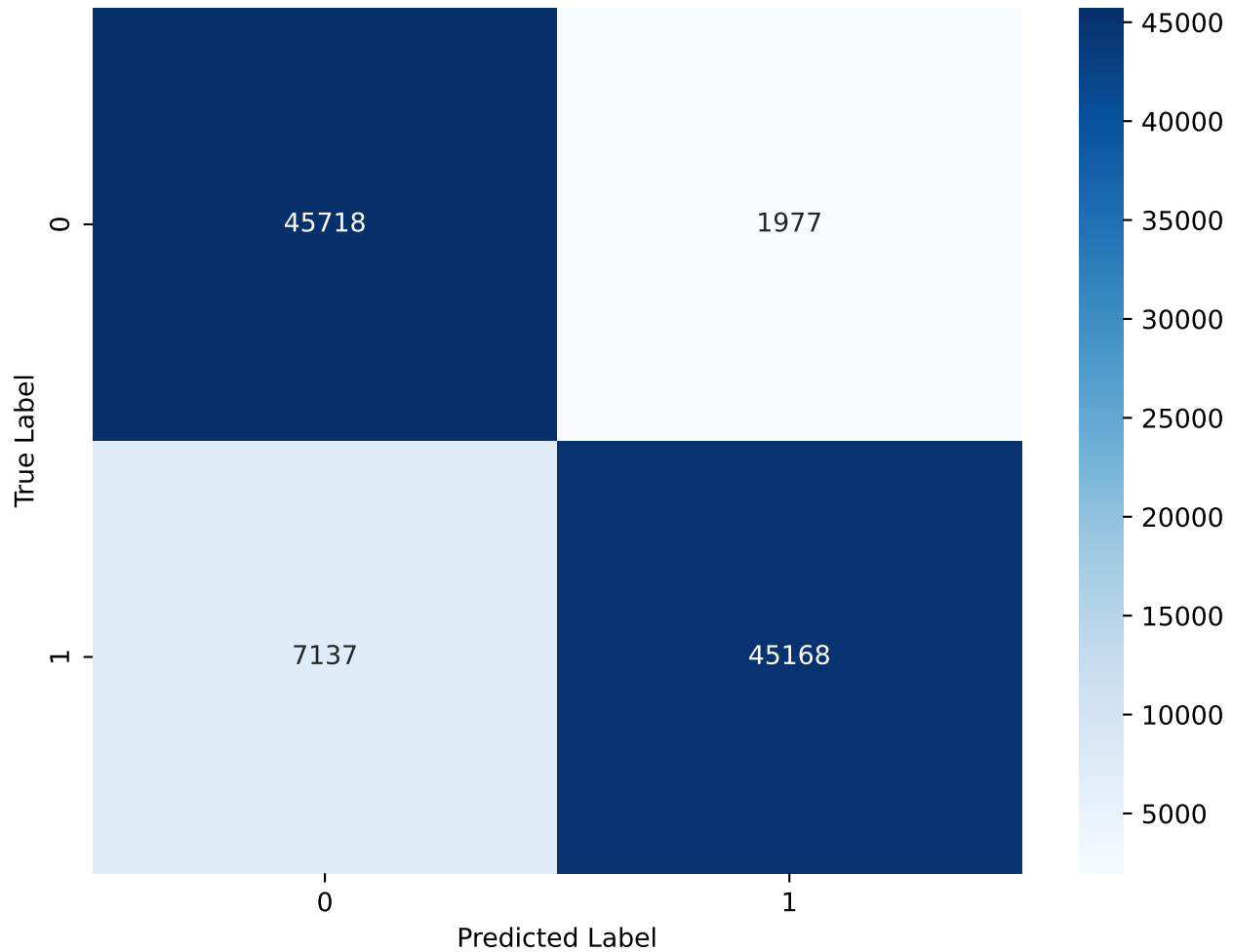
Confusion Matrix for E
