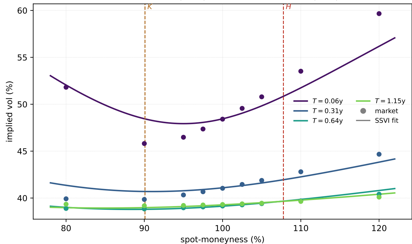
Calibrated SSVI (lines) vs raw market surface (dots)
