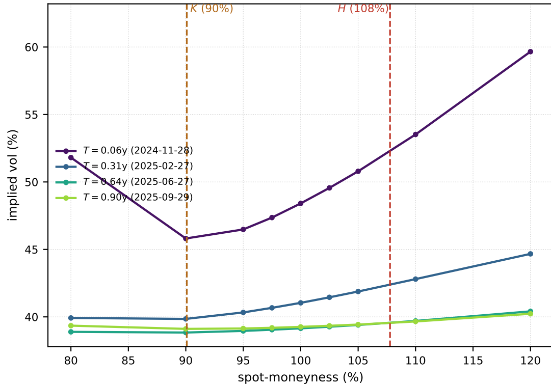
(b) smile slices; strike K and barrier H marked
