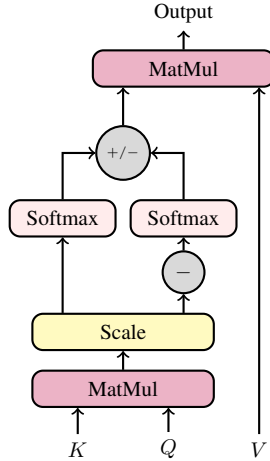
Figure 1: Signed Dual Attention block.
