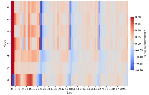
Figure 2: Autocorrelation Structure in ETTh2 Dataset.
