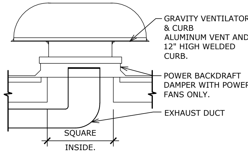
3 EXHAUST HOOD DETAIL SCALE: 1" = 1'-0"
