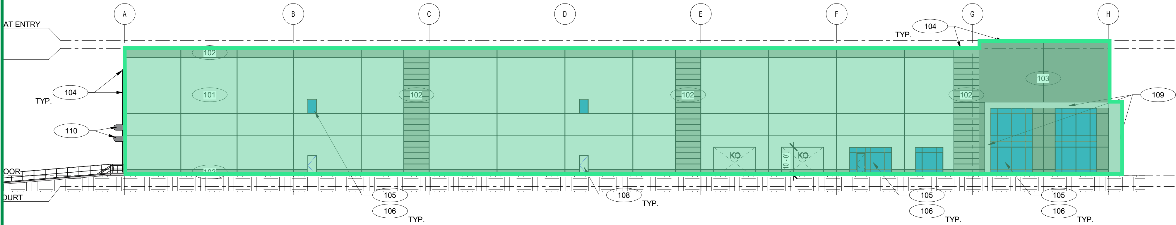
4 OVERALL WEST ELEVATION
