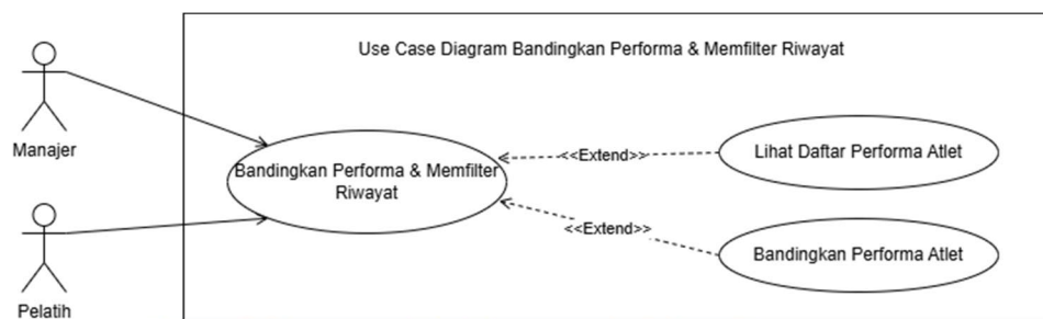
Gambar Use Case Diagram Bandingkan Performa & Memfilter Riwayat
