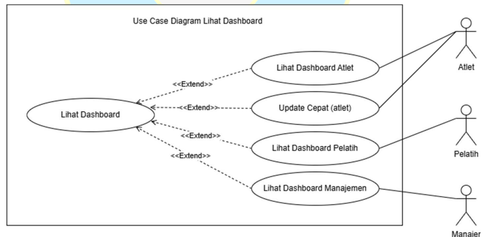
Gambar Use Case Diagram Lihat Dashboard
