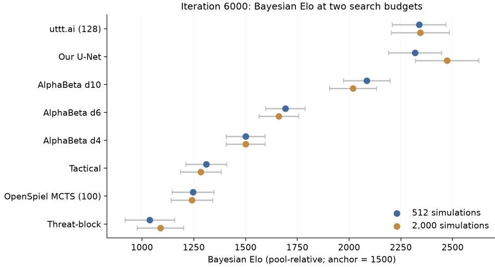
Fig. 3. Iteration 6000 rated in the same eight-entrant, 560-game pool at two search budgets, anchored at AlphaBeta d4 = 1500. Every opponent lands within a few Elo of its own rating in the other championship, so the pool itself has not moved; the agent alone does, by about 155 Elo, which is what makes the two separate fits comparable. At 512 simulations it sits just behind uttt.ai despite winning their head-to-head; at 2,000 it leads outright. Ratings are pool-local, not universal.
