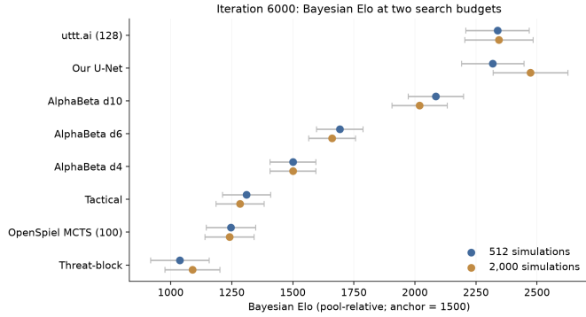
Fig. 4. Iteration 6000 rated in the same eight-entrant pool at two search budgets. Every opponent’s rating is essentially unchanged between the two championships, which is what makes the two fits comparable; the agent alone moves, by about 155 Elo.
