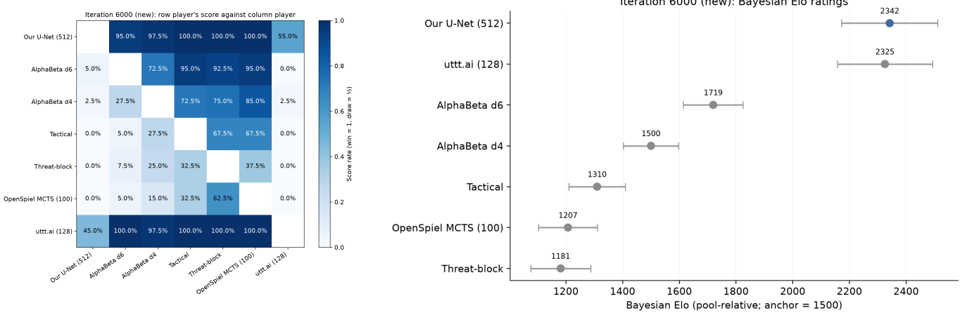
Fig. 3. Iteration-6000 championship. Left: round-robin score matrix (row player’s score against column player). Right: pool-local Bayesian-Elo ratings with 95% CIs, anchored at AlphaBeta d4 = 1500.
