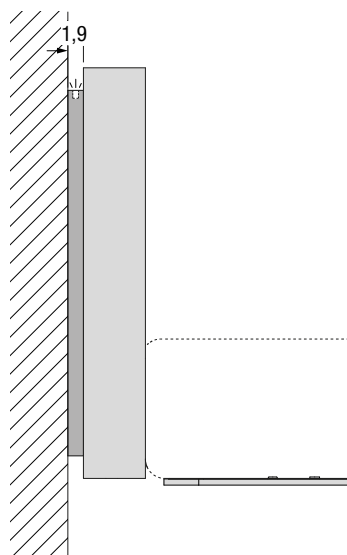
Imbottita con LED Upholstered with LED
