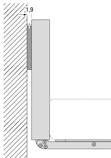
Imbottita con LED Upholstered with LED
