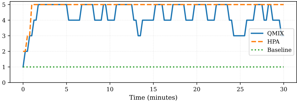
API Replicas
