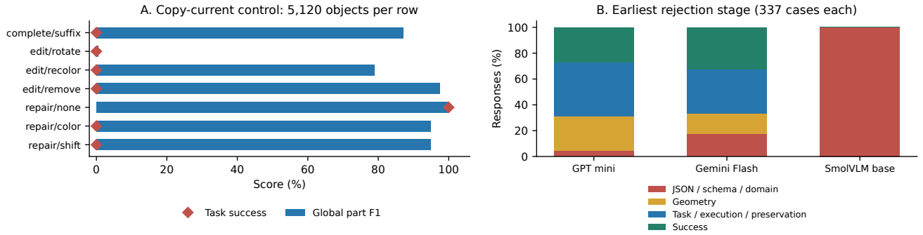
Figure 7. Previously measured no-operation and failure-stage diagnostics. The left panel uses the full casebank; the right uses the 337-case two-model/local-base study, not the new three-source matrix.
