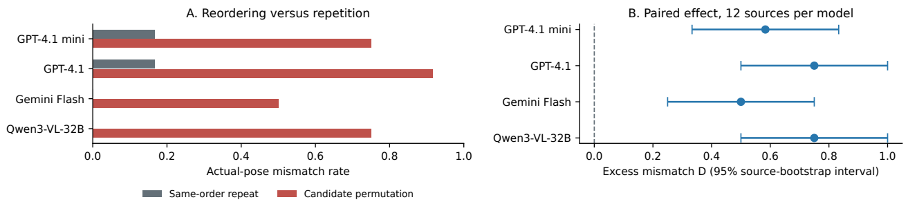
Figure 8. Measured same-order repetition versus candidate permutation on 12 shared development sources. Intervals resample source groups and do not constitute independent population confirmation.
