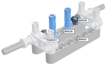
Subassembly B: 12 parts, original pose
