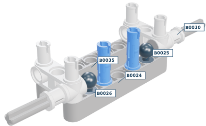
Subassembly A: 12 parts, original pose
