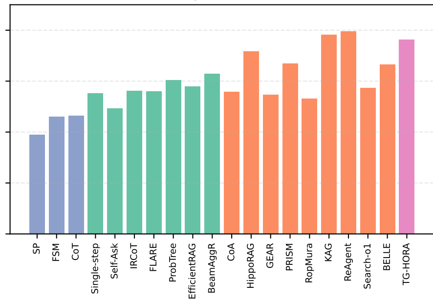
HotpotQA (F1)
