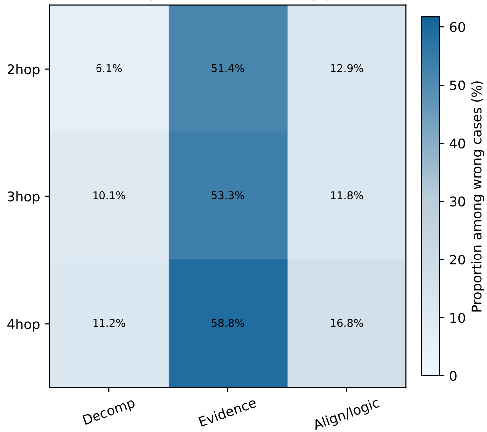
(b) Error composition within wrong predictions
