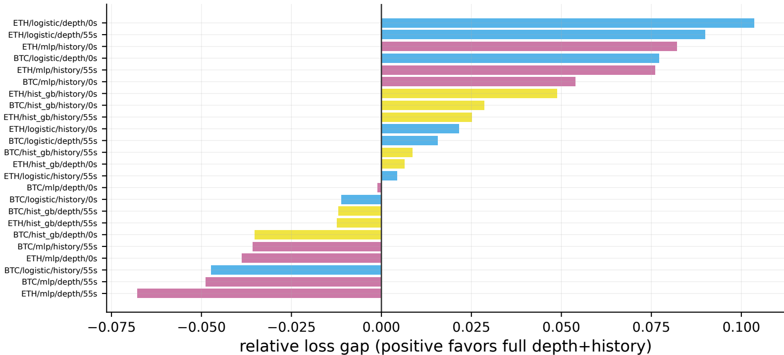
No common crossing: gaps change sign across model × asset × factor
