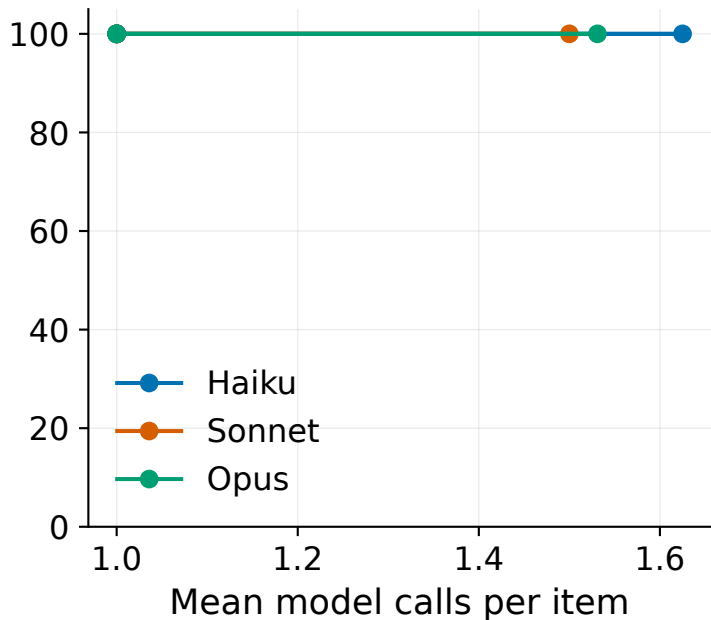
Clean completion (%)
