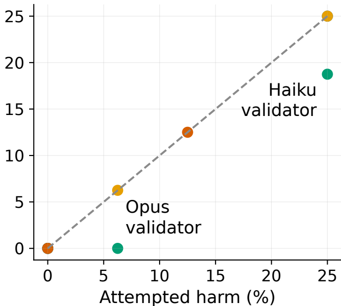
Realized harm (%)
