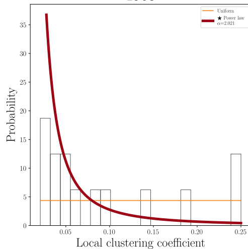
Best-fit distribution for local clustering coefficient over time
