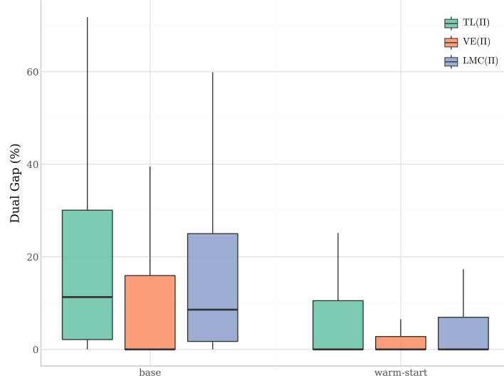
Figure 2: Dual gap at the end of the root node for each model.
