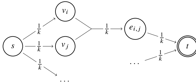
Figure 1: Problem \Pi_{\text{vc}} constructed from a VC instance.
