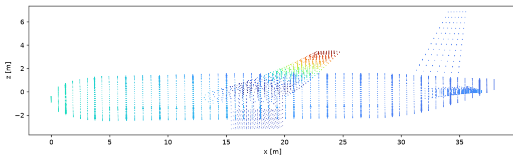
Mode 6, 2.25 Hz
