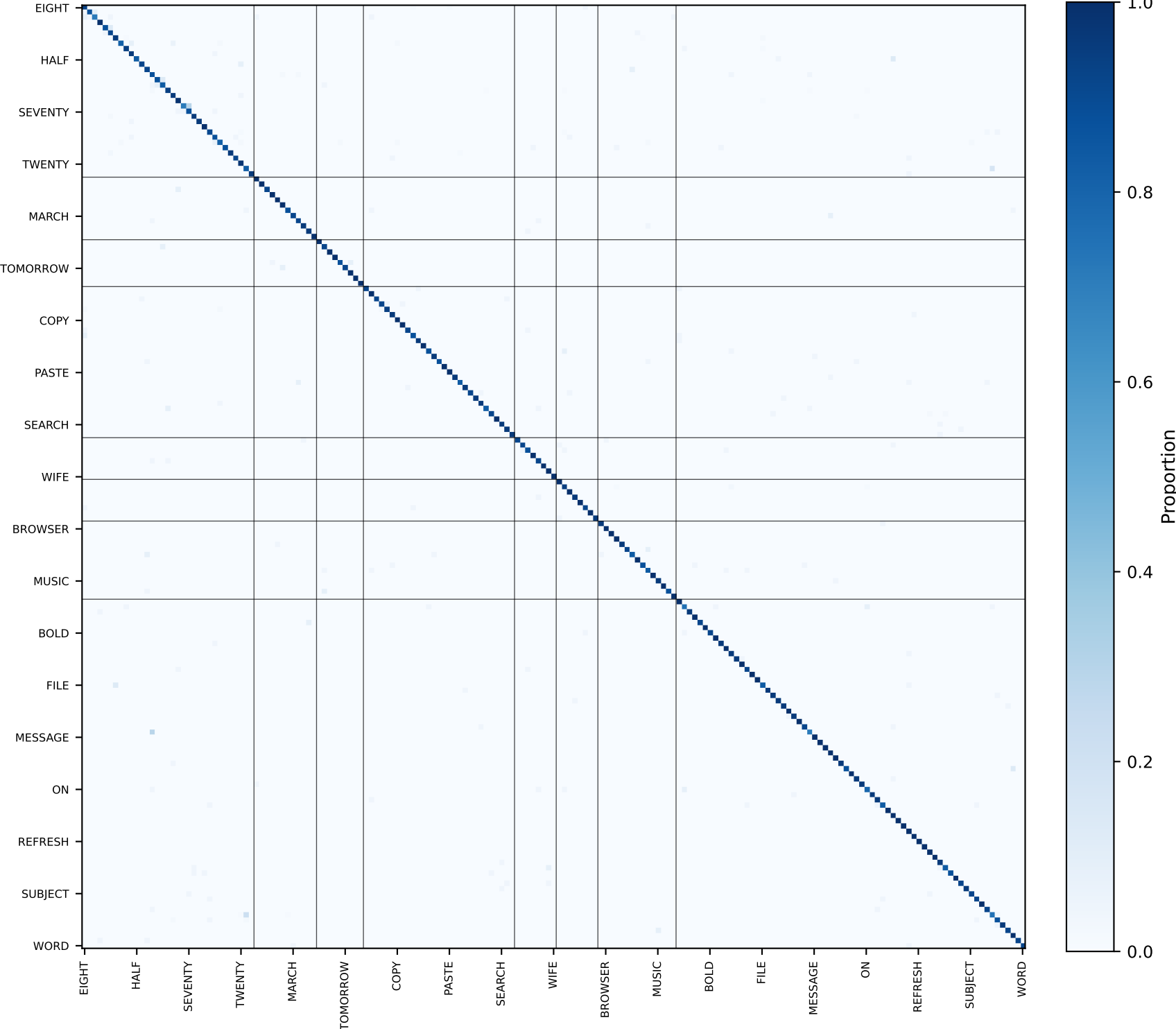
Confusion Matrix (row-normalized, sorted by phonetic category)
