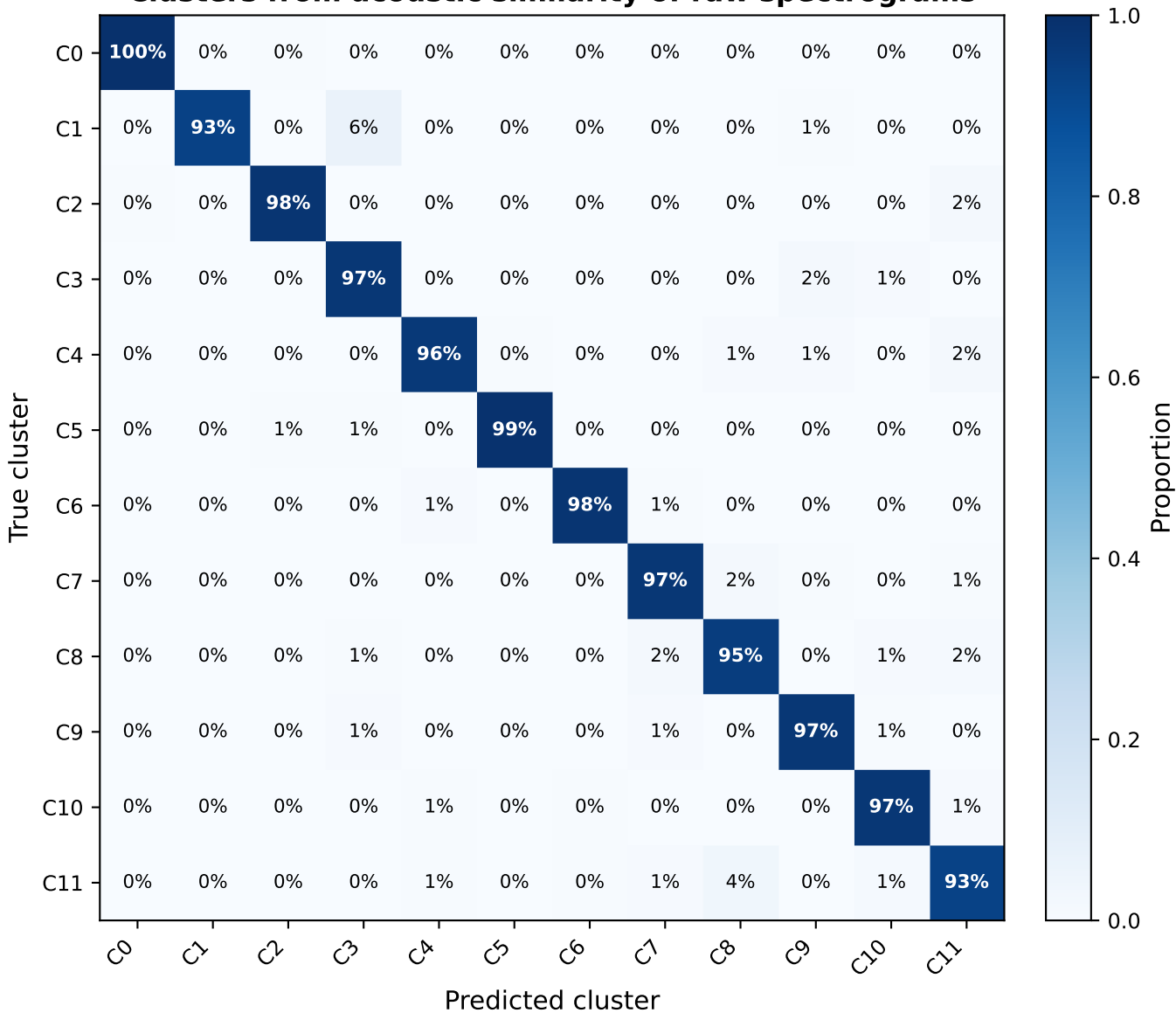
Cluster-Level Confusion Matrix (row-normalized) Clusters from acoustic similarity of raw spectrograms
