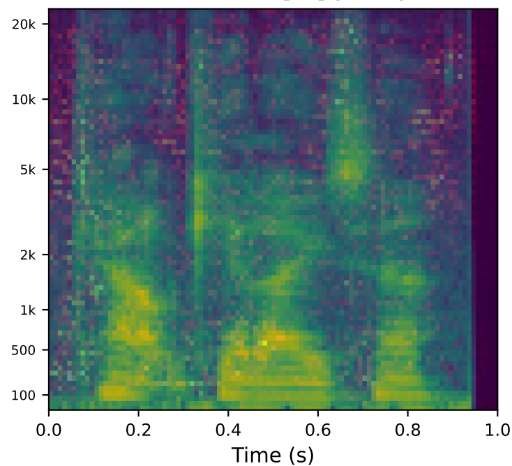
ATTACHMENT [C4] (96%)
