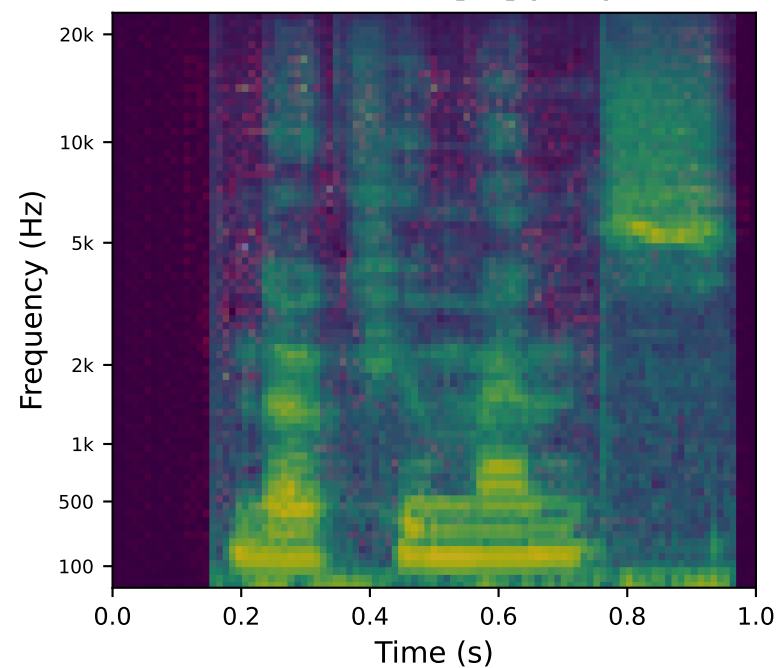
CALENDAR [C3] (99%)
