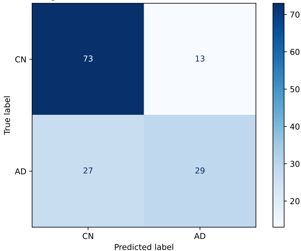
Average Test Set Confusion Matrix Across All Folds
