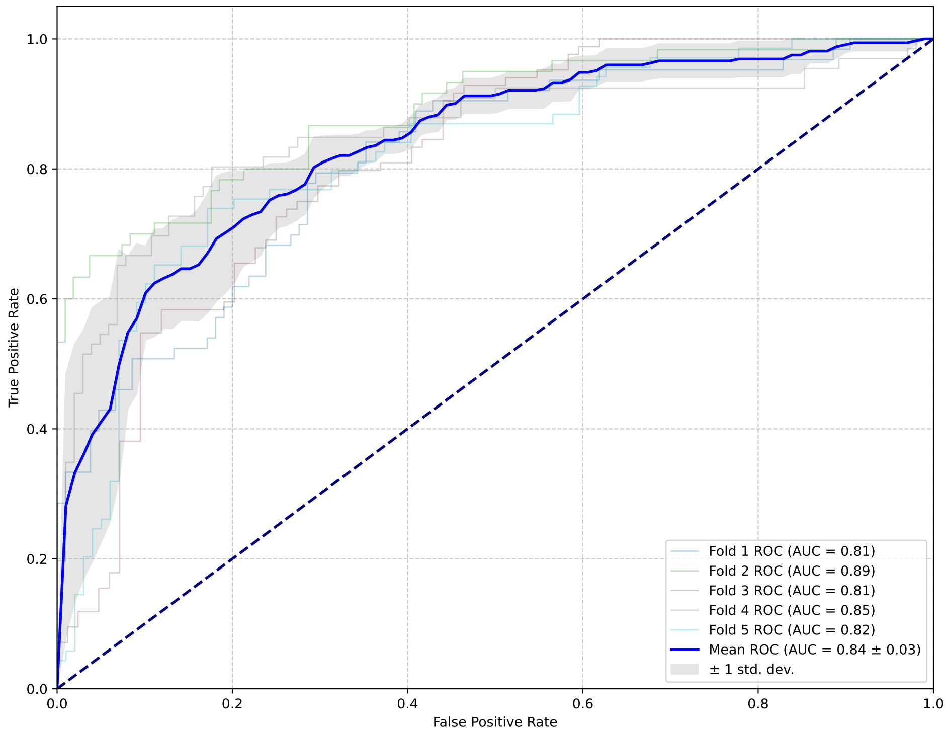
Cross-Validation ROC Curves
