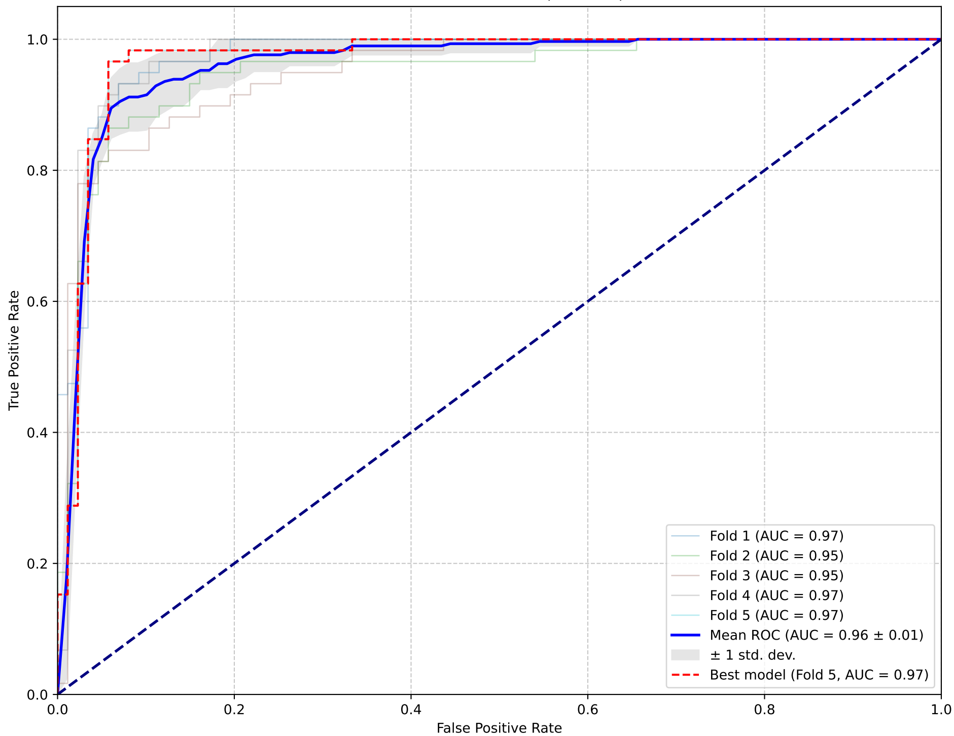
Test Set ROC Curves (All Folds)
