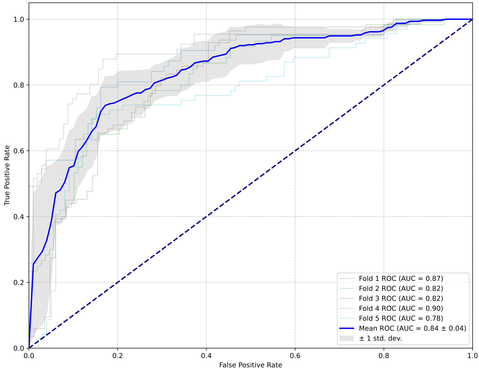
Cross-Validation ROC Curves
