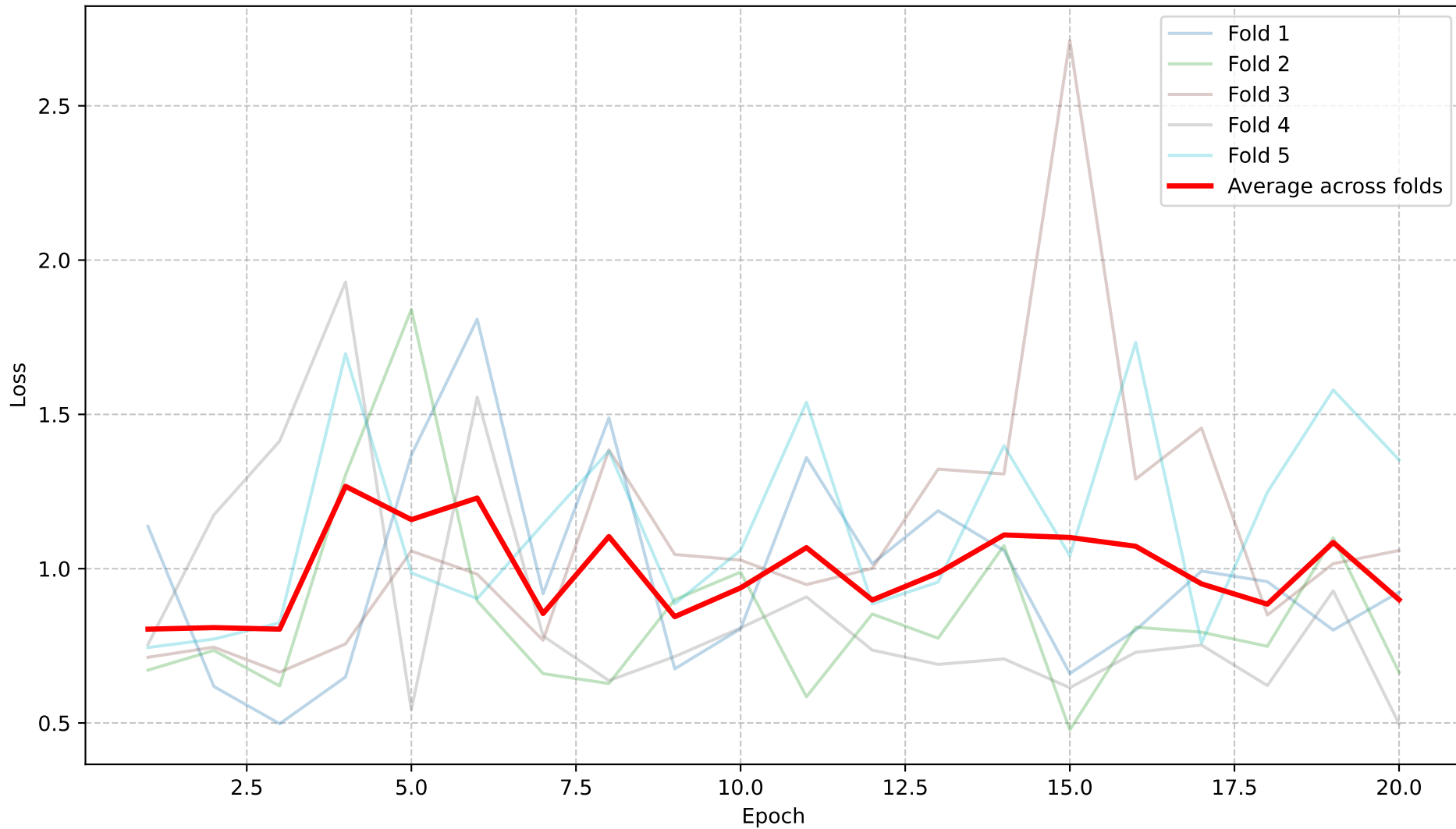
Validation Loss by Epoch
