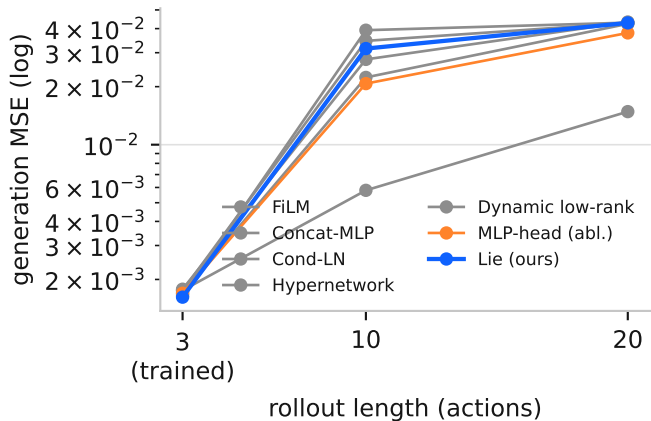
World-model rollouts: error compounds for
