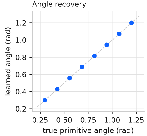
Figure 2: Left (S2): extrapolation to composition length 3 — conditions strictly longer than anything trained. Ours is flat at \sim 10^{-8} ; every baseline, including the identical-basis MLP-head ablation, degrades. Right (S1): learned singleton angles recover the true generators to 2 \times 10^{-4} rad — the operator is directly interpretable.
