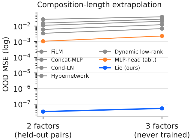
Figure 2: Left (S2): extrapolation to composition length 3 — conditions strictly longer than anything trained. Ours is flat at \sim 10^{-8} ; every baseline, including the identical-basis MLP-head ablation, degrades. Right (S1): learned singleton angles recover the true generators to 2 \times 10^{-4} rad — the operator is directly interpretable.
