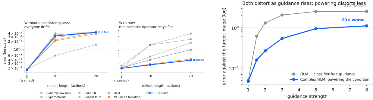
Figure 2: Left (S6, S6') : error against rollout length, trained only to length 3. Without a consistency loss every conditioner drifts at much the same rate. Adding one separates them: the isometric operator flattens out while the baselines keep climbing. Right (S8) : what turning guidance up does to the generated image. Both distort, since the target here is deterministic and there is no distribution to sharpen, but classifier-free guidance distorts twice as fast.
