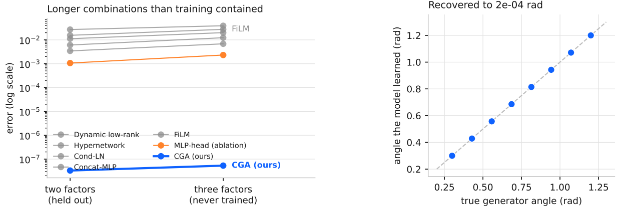
Figure 4: Left (S2): what happens when a test combination is longer than anything in training. Every baseline gets worse; CGA does not move, because composition is a property of its parametrization rather than something it had to learn. Right (S1): the angles the model learned for each condition, against the true generators of the data. Reading the weights tells you which plane a condition rotates, and how fast.
